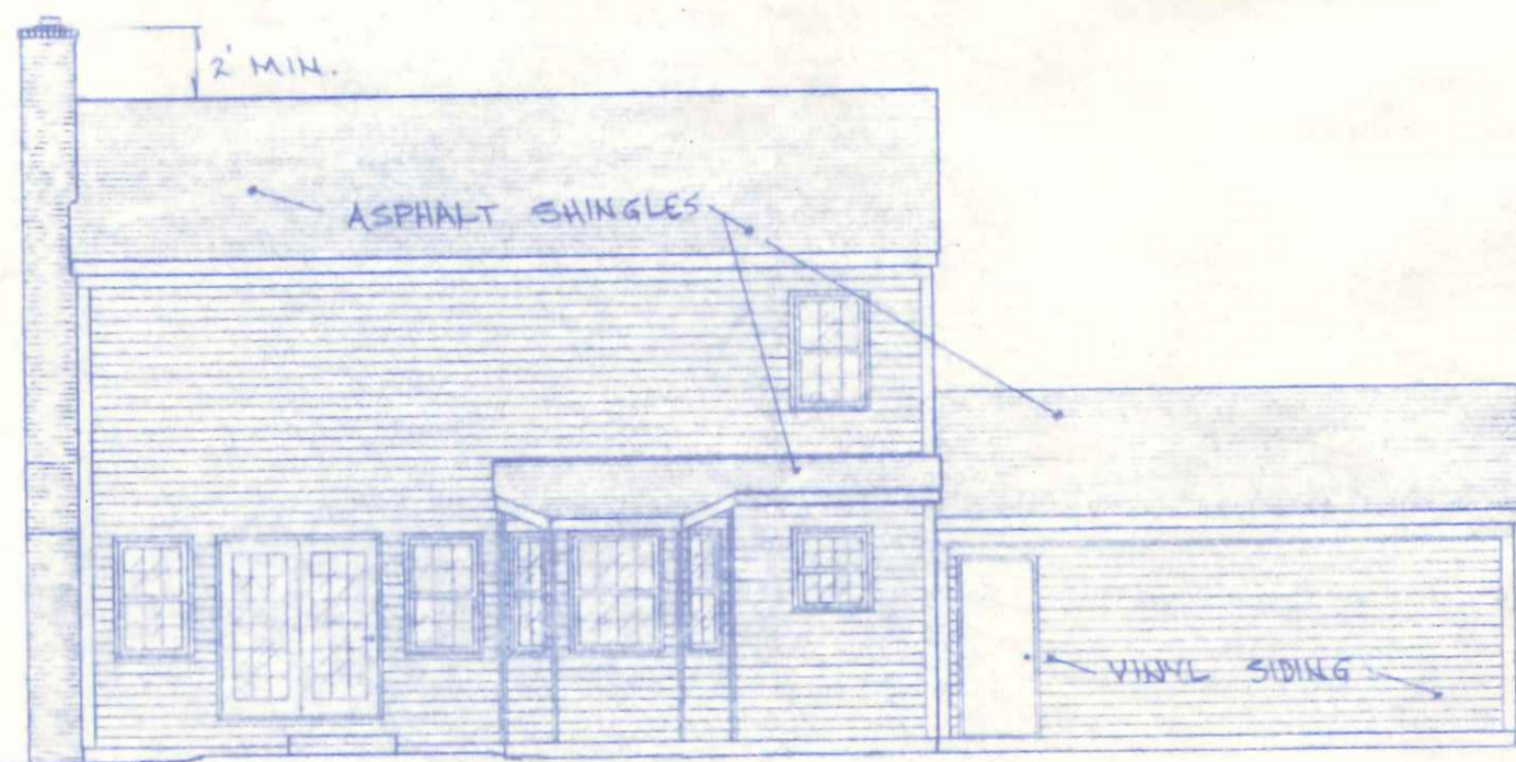
REAR ELEVATION 1/8" = 1'-0"
