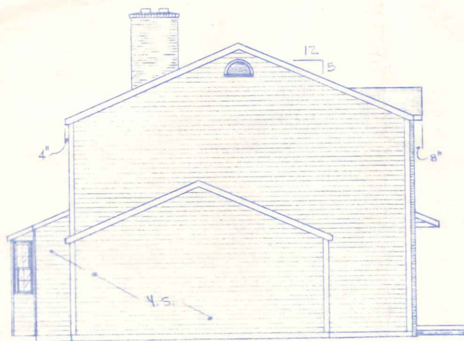
LEFT SIDE ELEVATION 1/8" = 1'-0"
