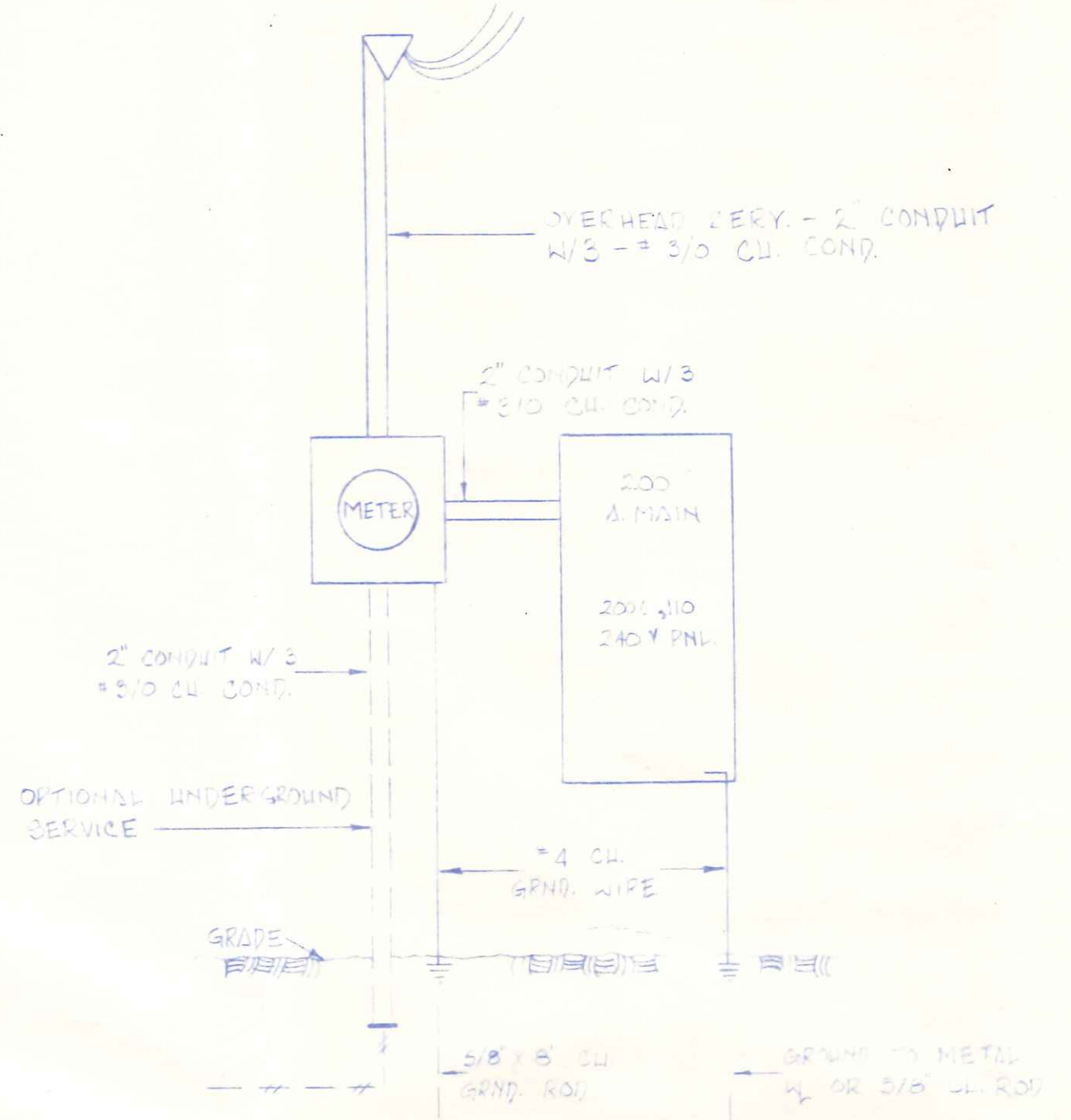
ELECTRICAL SERVICE DIAGRAM
