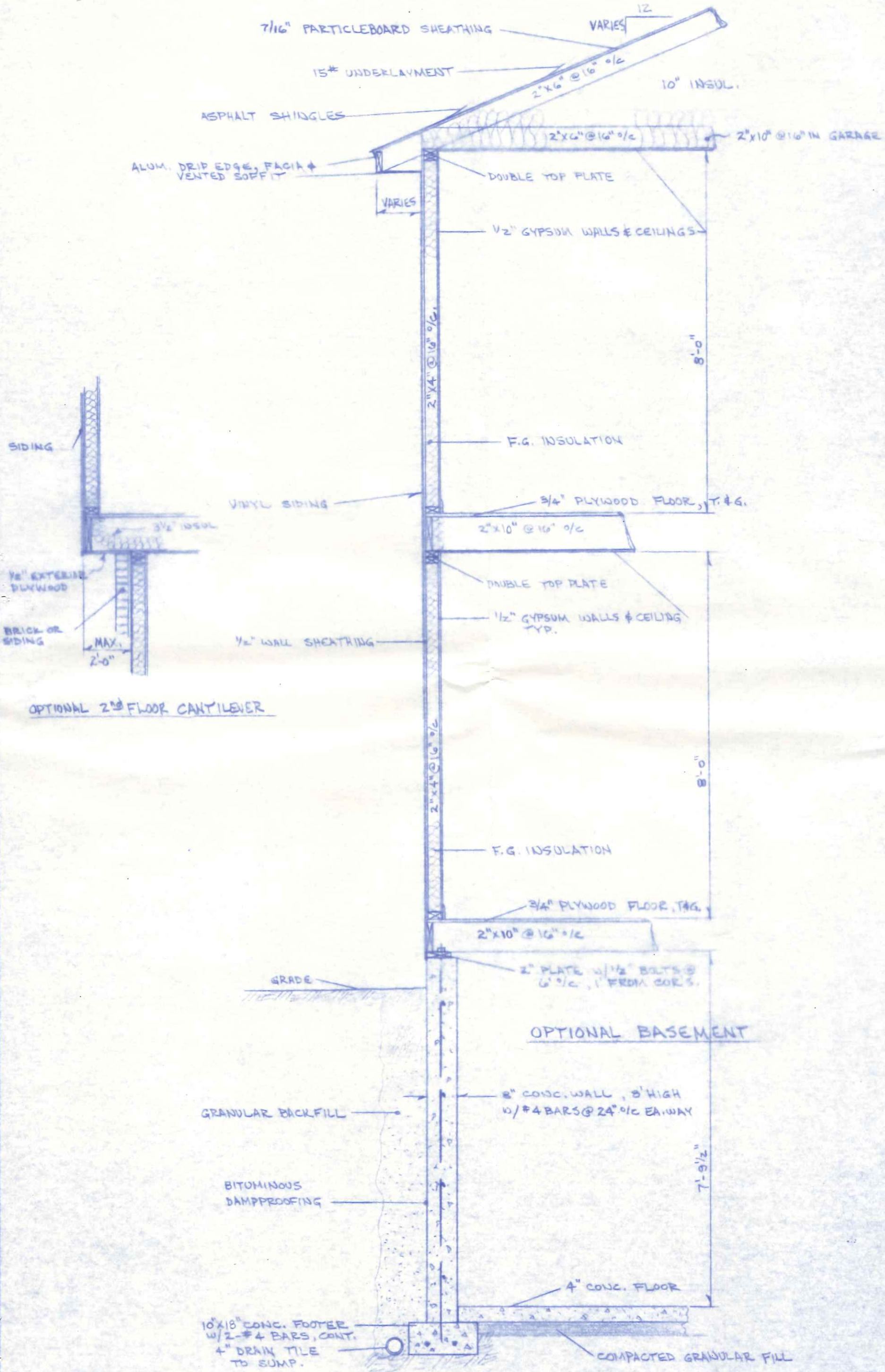
TYPICAL SECTION 2 STORY W/BASEMENT 1/2" = 1'-0" BECK CONSTRUCTION CO. AUG. 1986 R.D.S.
